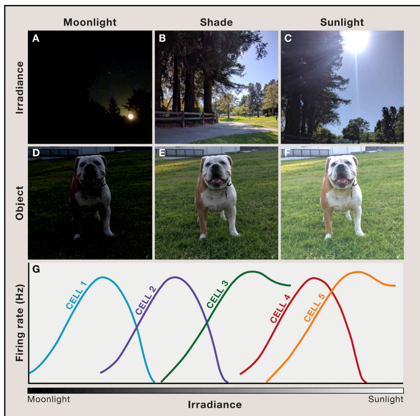
Figure 1. M1 ipRGCs Fire Selectively at Specific Irradiances
